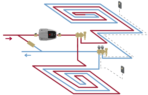
Underfloor heating system
